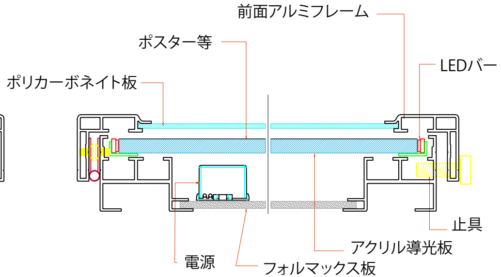
Section B-B Scale 1 : 1
