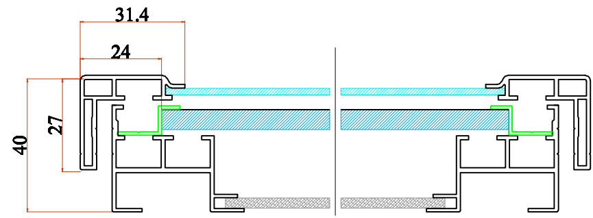
BR-SO40 Assembly Non-Scale
