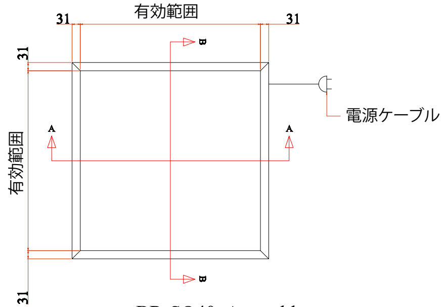
BR-SO40 Assembly Non-Scale
