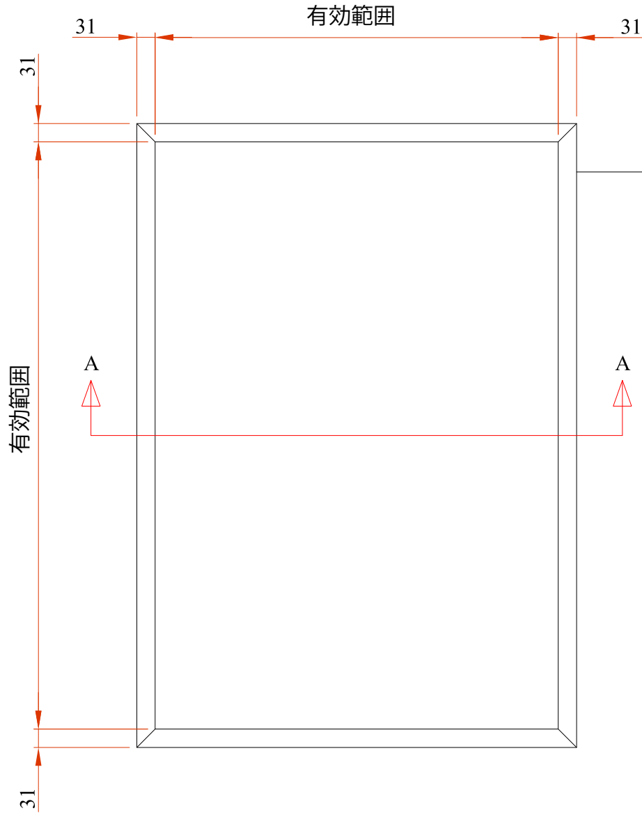
BR-SL70 Assembly Non-Scale
