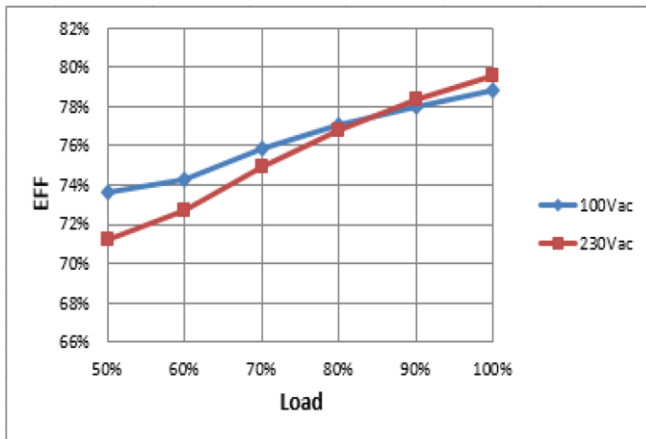
EFF VS. 負荷曲線 (300mA for ref.)
